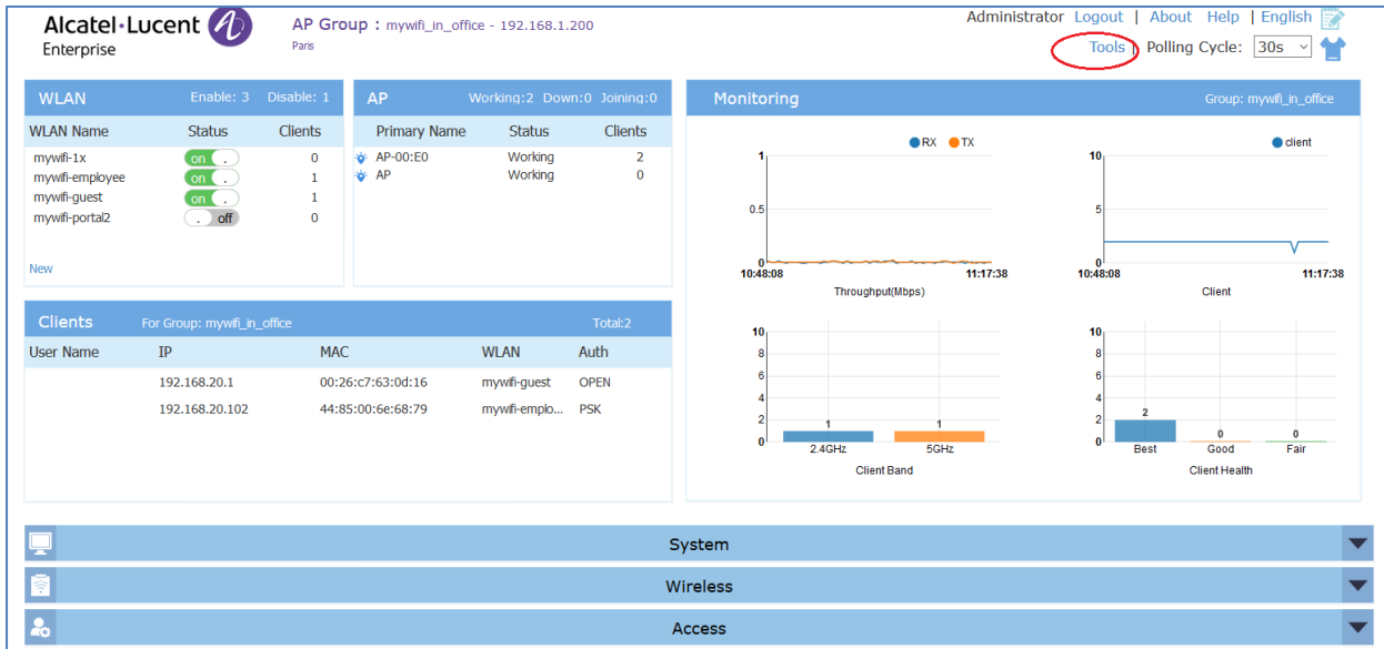
Figure 8-1 Tools in Dashboard
